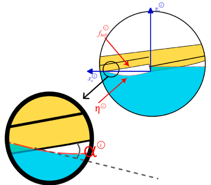
Fig. 20. Water surface profile behind a step and the local coordinate system used to find the ventilation length. The concept of local trim angle is also illustrated in a zoomed-up view.
